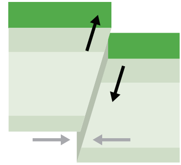
FAILLE INVERSE
