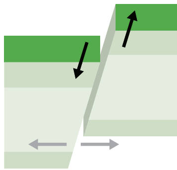
FAILLE NORMALE
